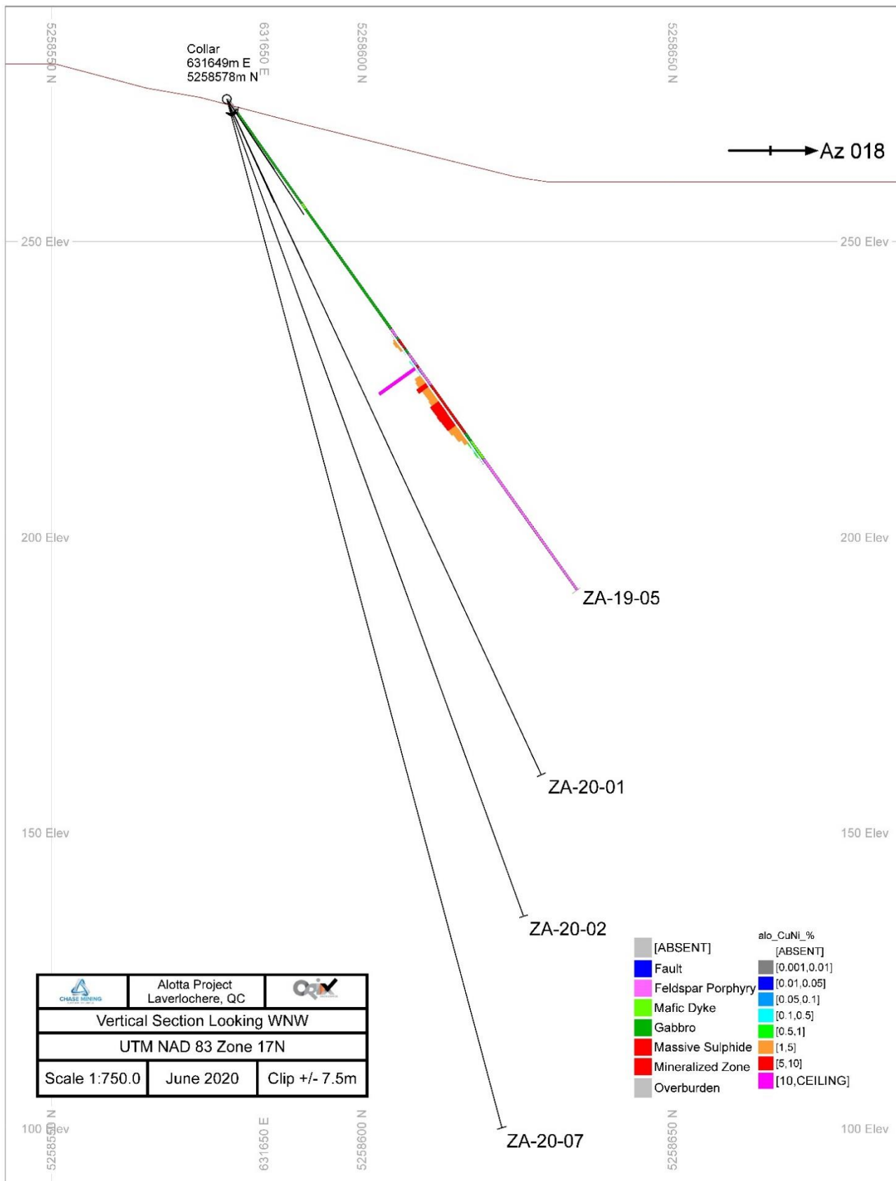
Figure 2: Vertical section looking WNW showing current hole ZA-20-01 and the Hole ZA-19-05 target zone of mineralisation
