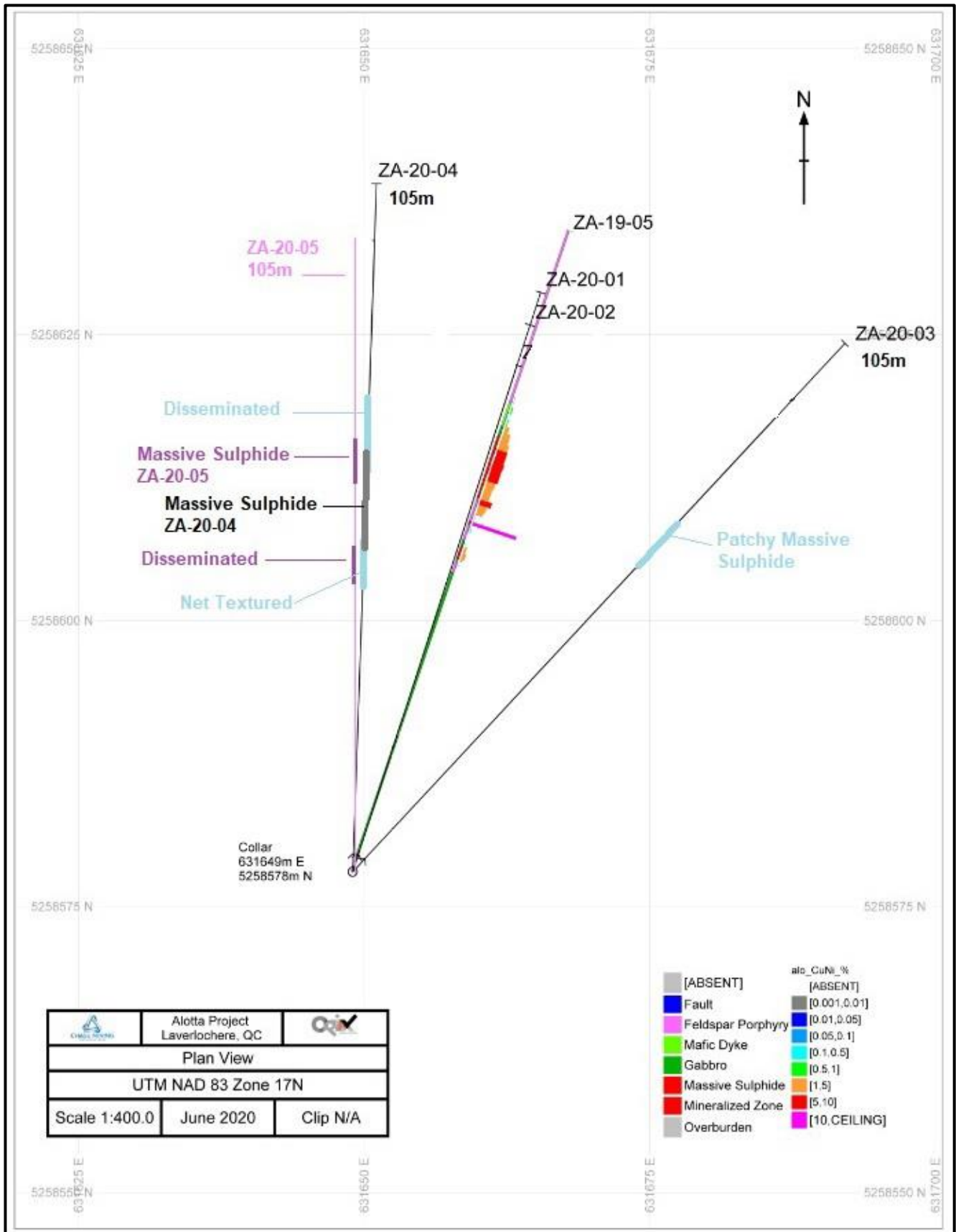
Figure 3: Schematic Plan View of Hole ZA-20-05, an undercut of ZA-20-04.
